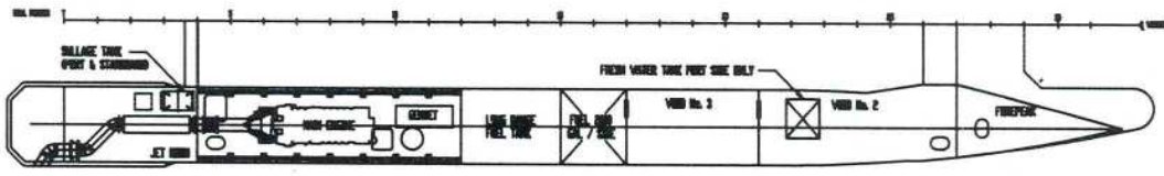
PLAN BELOW DECK
