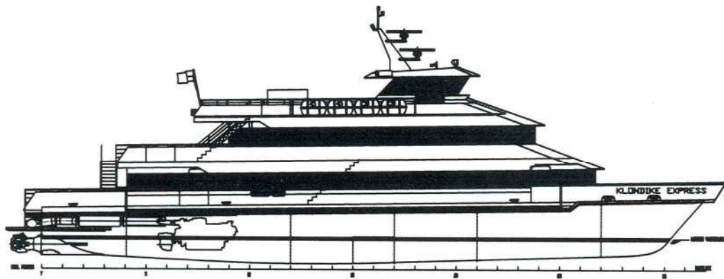
OUTBOARD PROFILE
