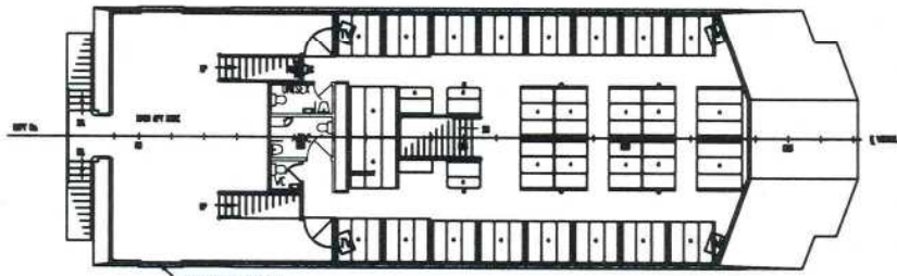
PLAN OF UPPER PASSENGER DECK
