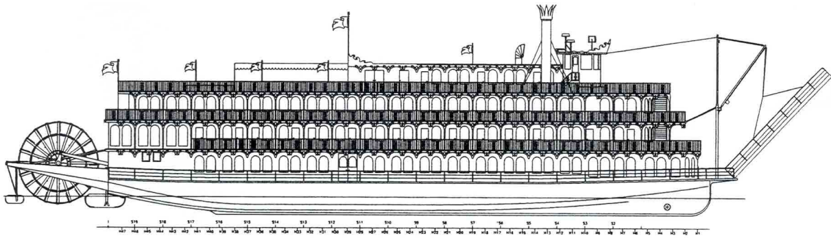
OUTBOARD PROFILE
