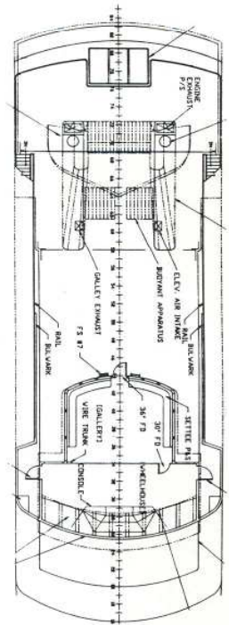
BRIDGE DECK
