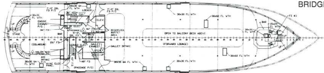
BALCONY DECK
