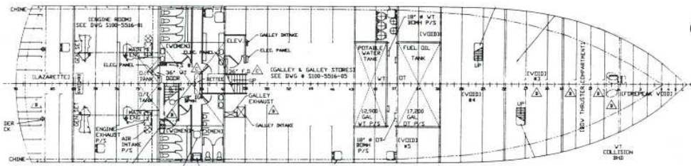
HOLD DECK
