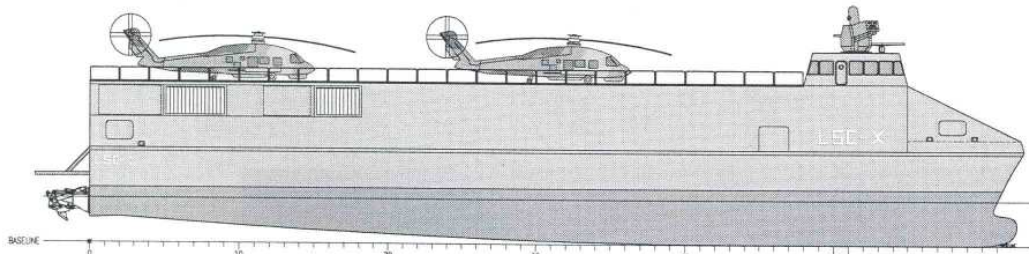
OUTBOARD PROFILE
