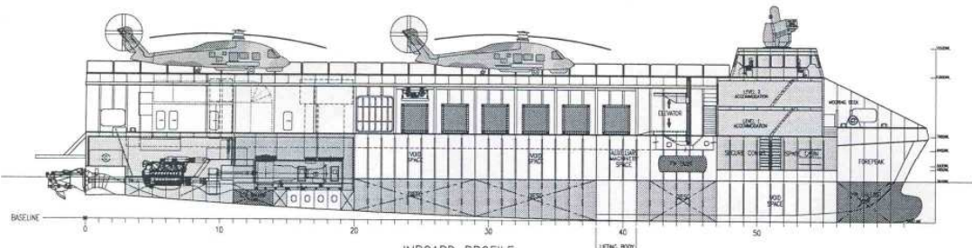
INBOARD PROFILE
