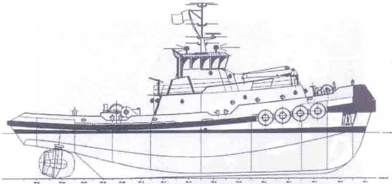
OUTBOARD PROFILE
