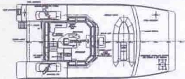
BRIDGE DECK PLAN
