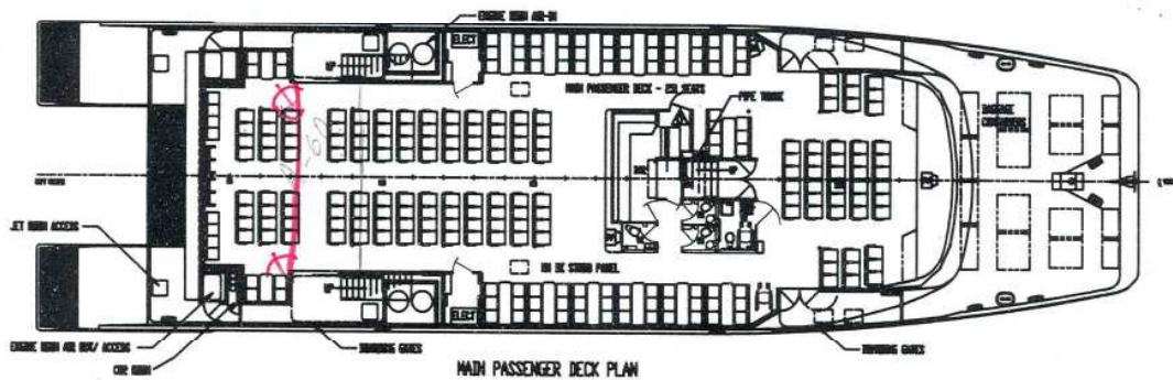
MAIN PASSENGER DECK PLAN
