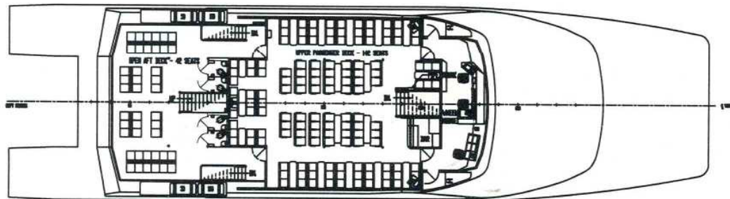
UPPER PASSENGER DECK PLAN
