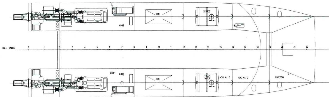
PLAN BELOW DECK
